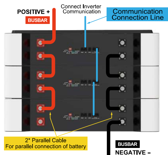
Schematic Diagram of Connection and Use Of Three Battery
