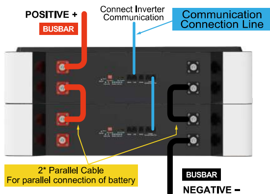
Schematic Diagram of Connection and Use Of Two Battery
