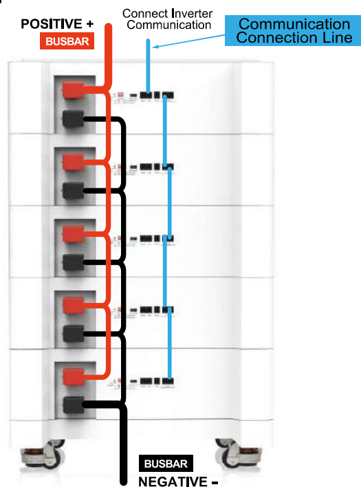
Schematic Diagram of Connection and Use Of Five Battery
