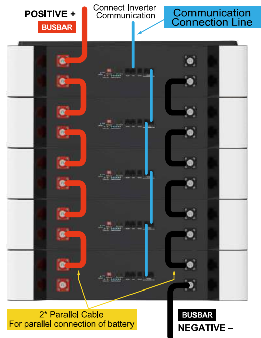
Schematic Diagram of Connection and Use Of Five Battery
